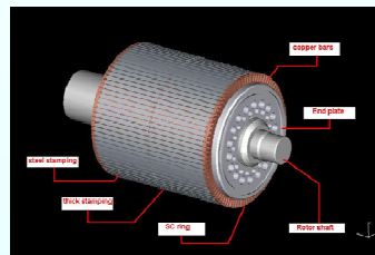
FEM for Analyzing the Traction Motor Rotor Bar Crack
