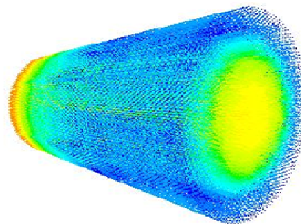
Checking of Smooth Flow of Duct for a Steam Boiler ( CFD Analysis )
