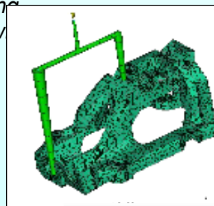
Mold Flow Analysis of Shifter Box
